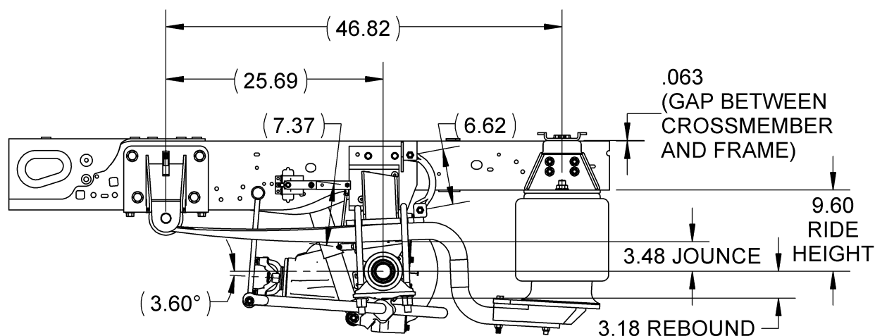
Figure 1: Suspension range of motion
