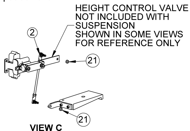
Figure 7: Detailed exploded views "A", "B" and "C"
