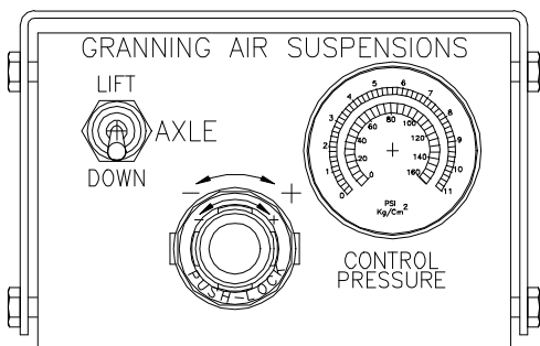
Figure 5 - Control Panel
