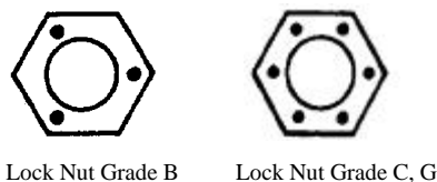
Grade Markings on Locknuts
